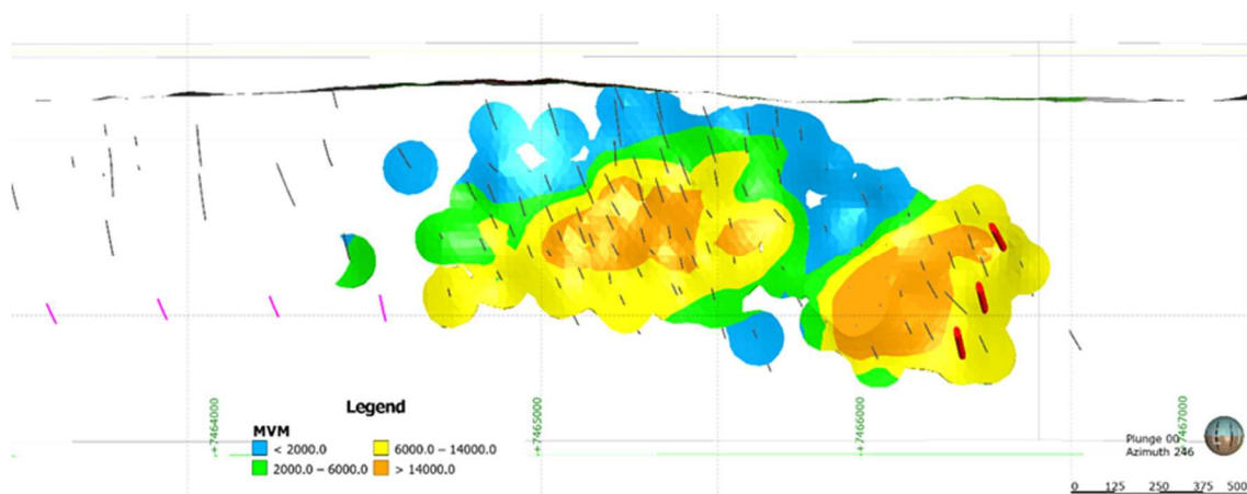
Figure 10: West looking longitudinal section view of Nautanen. Contours show copper percent multiplied by width of intersection (MVM). Red pierce points show the extension holes drilled in early 2020. Purple pierce points are the holes that were planned but postponed. Back pierce points are previous drilling.
