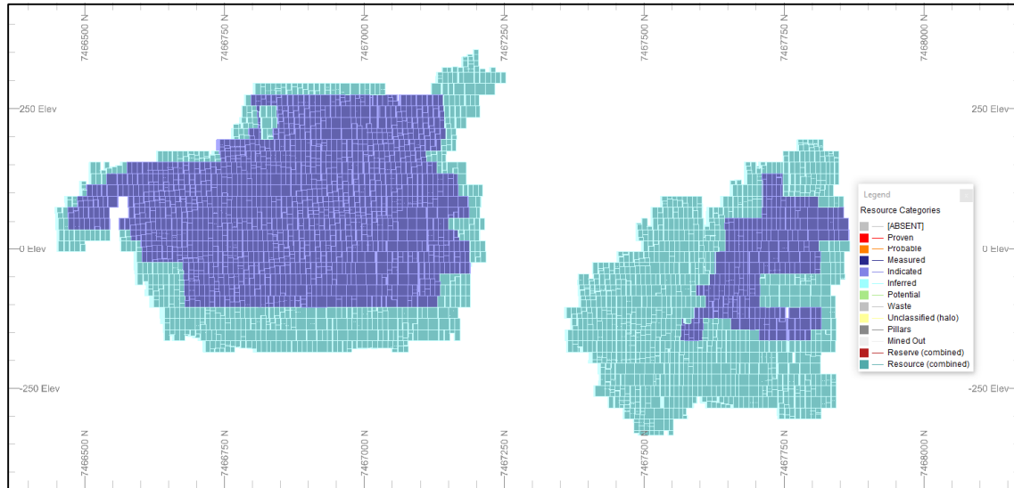
Figure 11. North (right) – south (left) longsection view of the classified Nautanen block model (blue: Indicated; cyan: Inferred).
