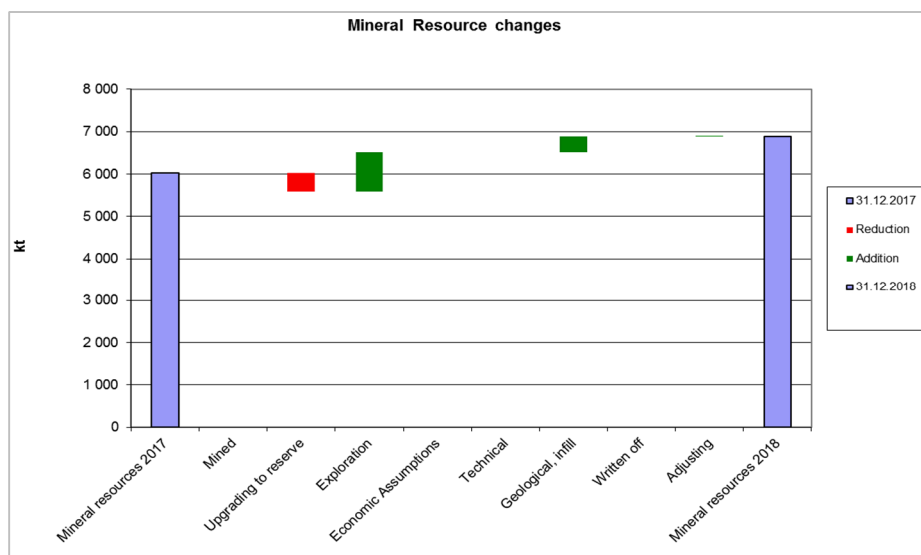
Figure 24. Graphic explanation of changes to the mineral resource at Kylylahti
