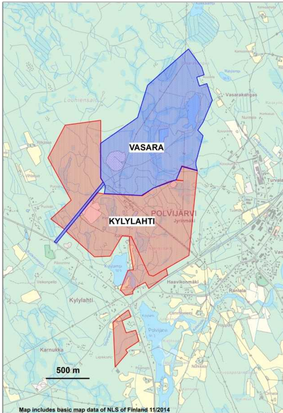
Figure 4. Map showing Kylylahti (Boliden) and Vasara (Mondo) mining licenses
