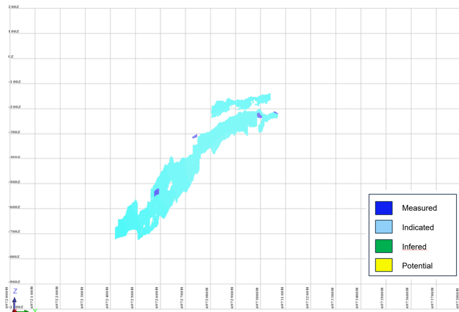
Figure 19. Schematic long section of mineral resource classification of cobalt domains at Kylylahti
