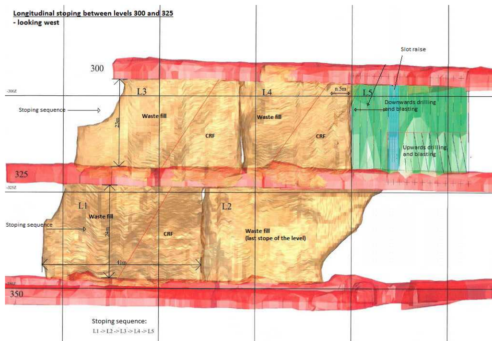
Figure 12. Example of longitudinal stoping.
