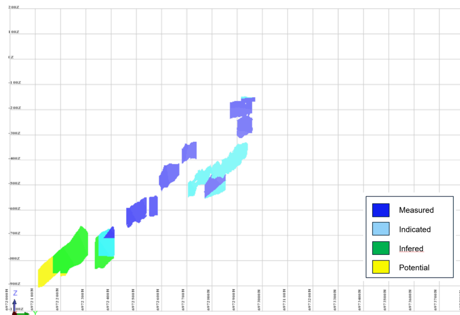
Figure 20. Schematic long section of mineral resource classification of nickel domains at Kylylahti
