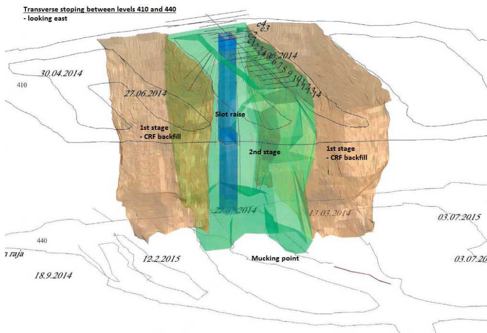
Figure 11. Example of secondary transverse stoping.
