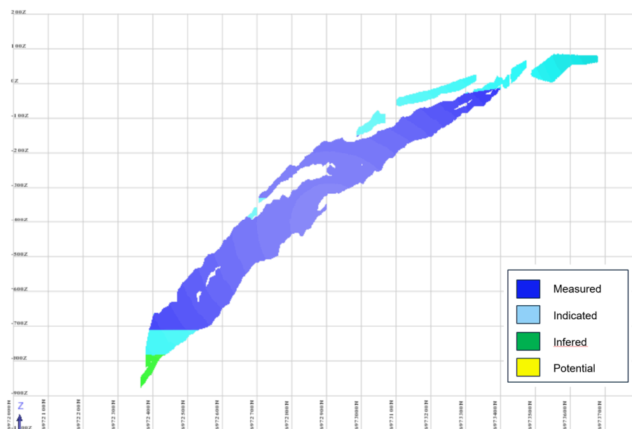
Figure 17. Schematic long section of mineral resource classification of copper domains at Kylylahti.
