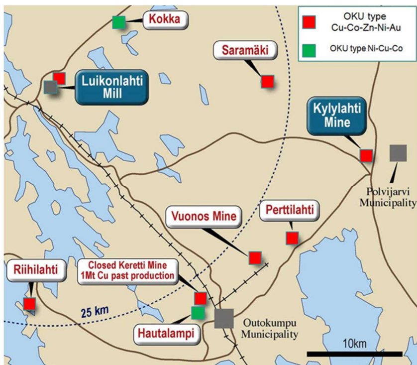
Figure 3. Map of the Outokumpu area showing the location of the mine and mill
