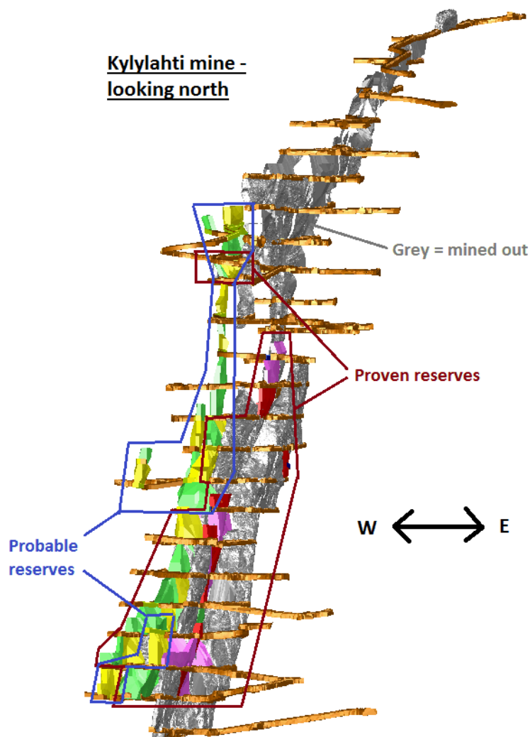
Figure 22. Location of proven and probable mineral reserves at Kylylahti mine with December 2018 reserve planned and mined out stopes as a background – looking north.
