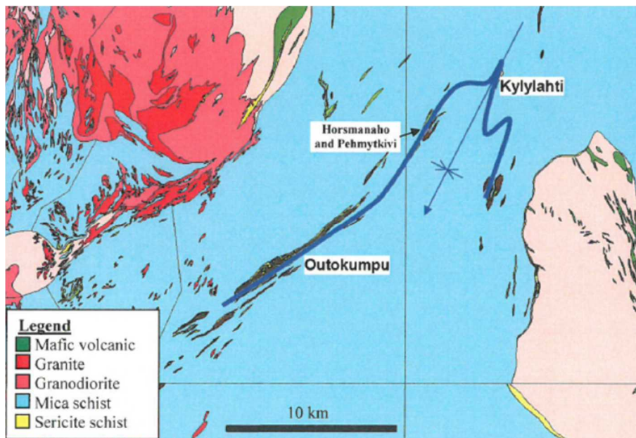
Figure 7. Geology plan showing the location of the Kylylahti deposit in the nose of the regional synform that hosts the Outokumpu district. Blue lines show simplified trace of the synform.
