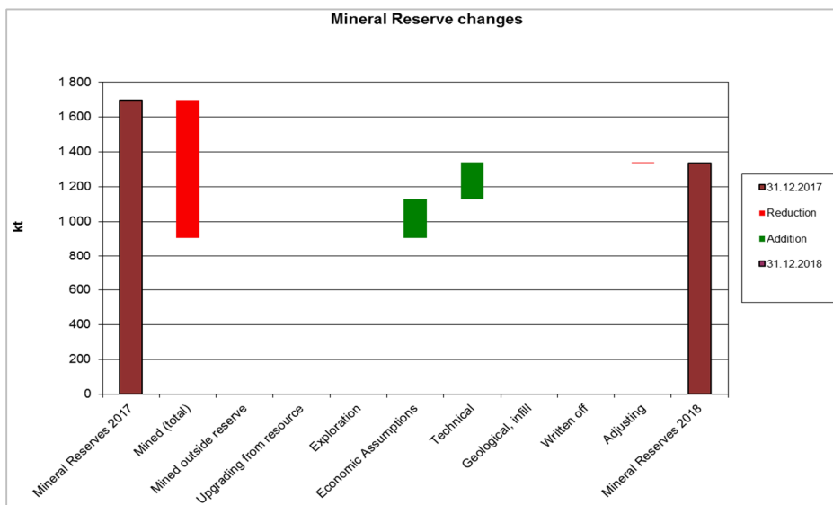
Figure 23. Graphic showing changes in Kylylahti's total mineral reserve from 2017 to 2018.
