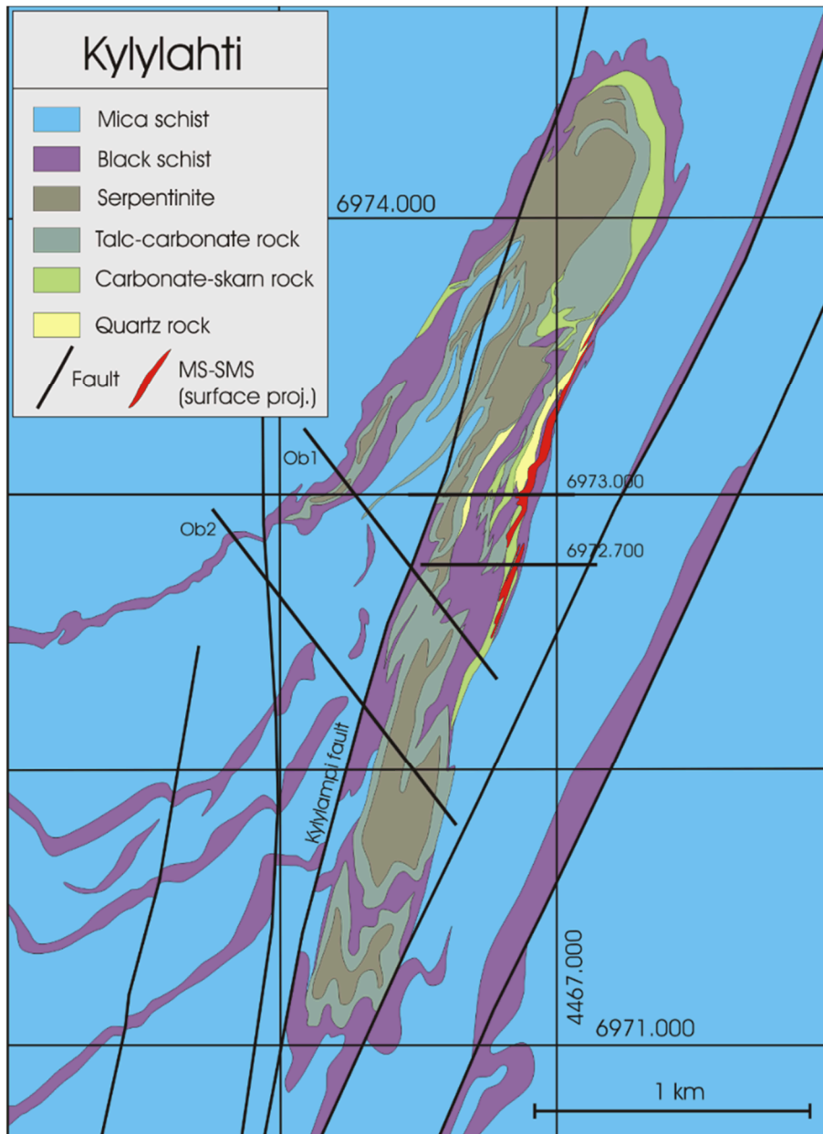
Figure 8. Kylylahti complex, showing surface projection of the massive-semimassive sulphide mineralization. Picture from Kontinen et al. (2006).
