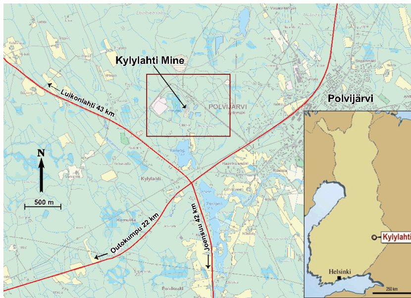
Figure 2. Location map for the Kylylahti mine. Map includes basec map data of NLS of Finland 11/2014
