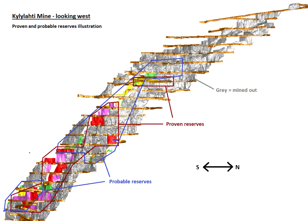
Figure 21. Location of proven and probable mineral reserves at Kylylahti mine with December 2018 reserve planned and mined out stopes as a background – looking west
