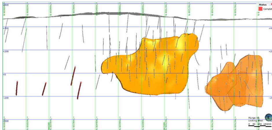
Figure 9 West looking longitudinal section view of Nautanen. Orange wireframes show the 2020 mineral resource. Red pierce points show the holes drilled in 2021.
