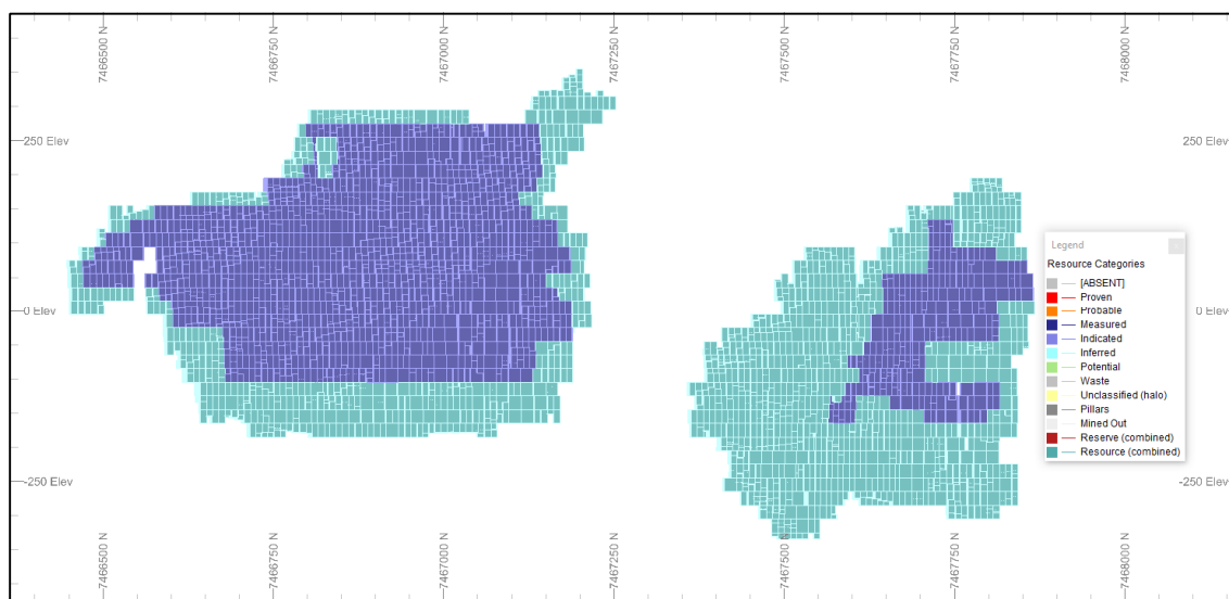
Figure 10. North (right) – south (left) longsection view of the classified Nautanen block model (blue: Indicated; cyan: Inferred).
