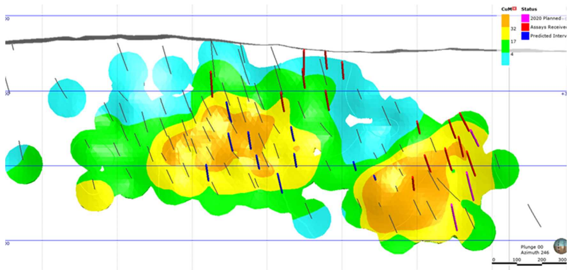
Figure 9. West looking longitudinal section view of Nautanen. Contours show copper percent multiplied by width of intersection. Red pierce points show 2019 drillholes with assays received. Blue pierce points show 2019 drillholes with predicted grades. Magenta pierce points show 2019 drillholes which will be completed in 2020.
