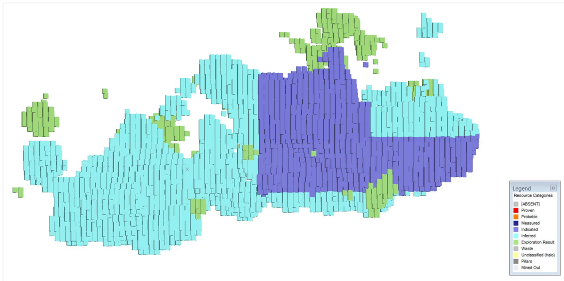
Figure 9. North (left) – south (right) longsection view of the classified Nautanen block model (blue: Indicated; cyan: Inferred; green: geol. potential).
