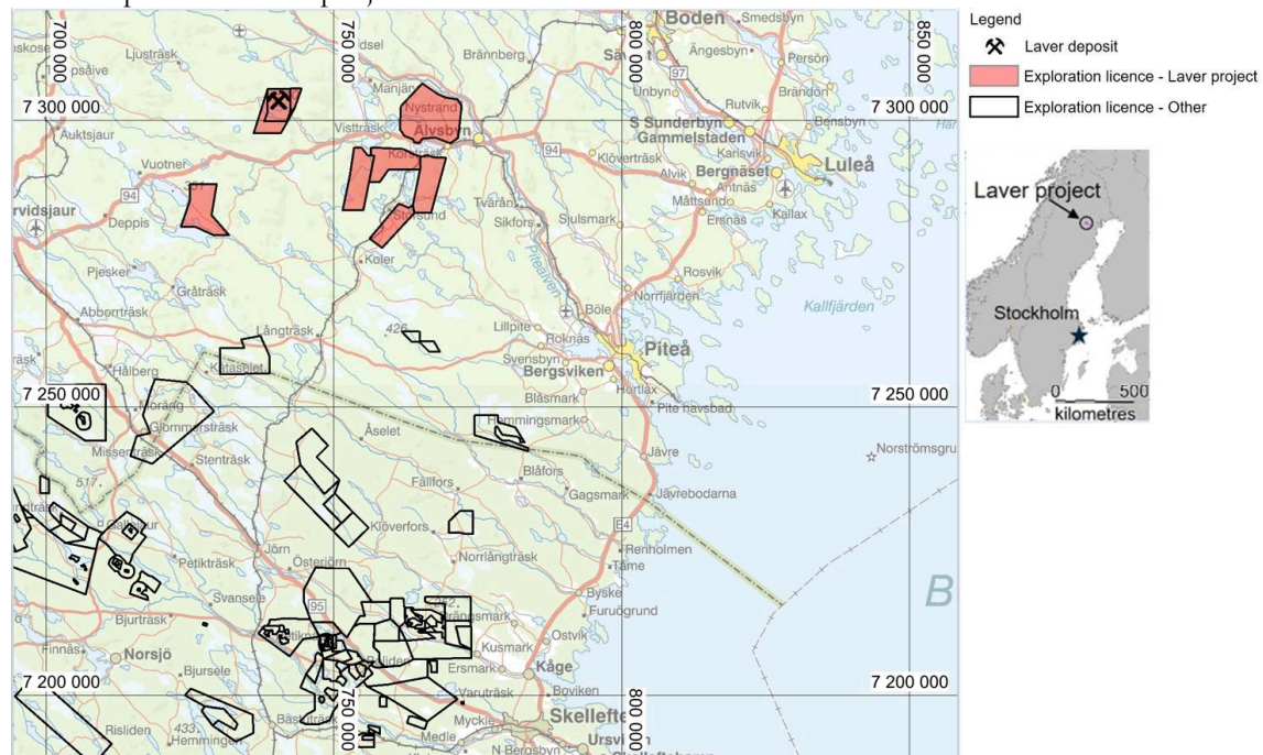
Figure 2 Location map of the Laver project. Coordinate system is SWEREF99TM (meters).
