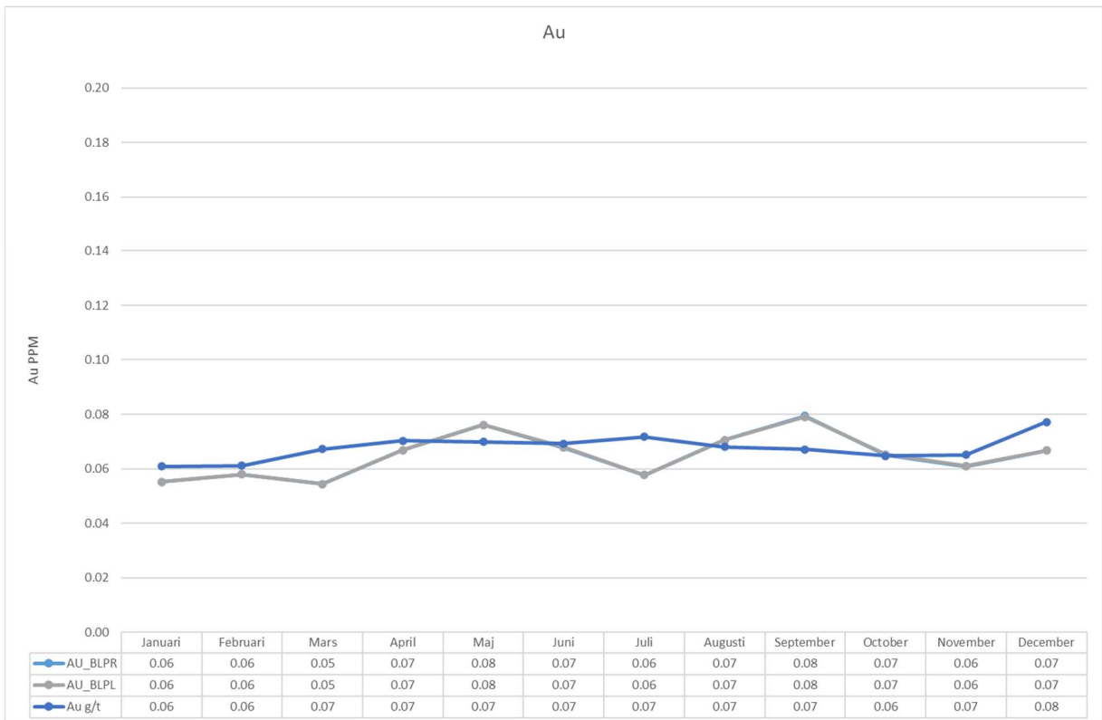
Figure 12: Comparing measured gold results from the processing plant with calculated results from the block models for gold.
