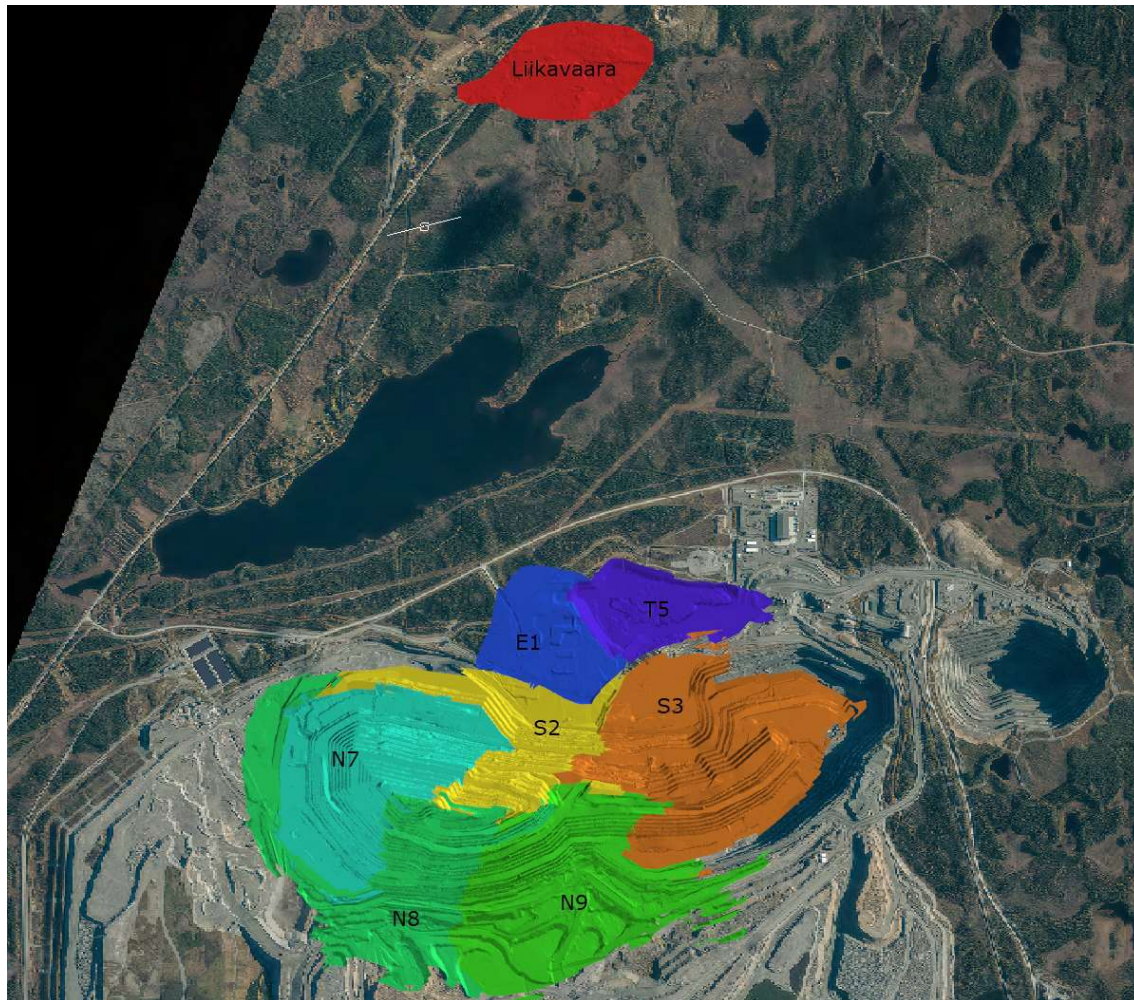
Figure 9. Overview of planned and active pushbacks at Aitik.
