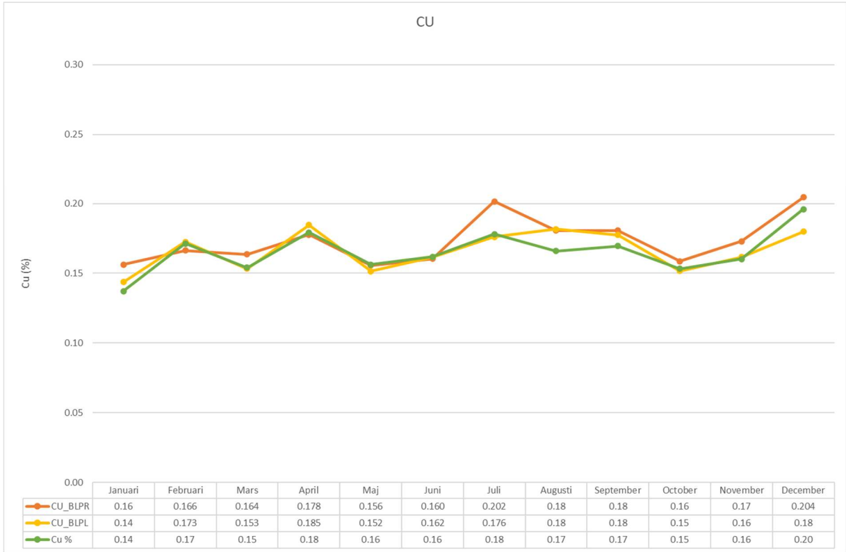
Figure 11: Comparing measured copper results from the processing plant with calculated results from the block models for copper.
