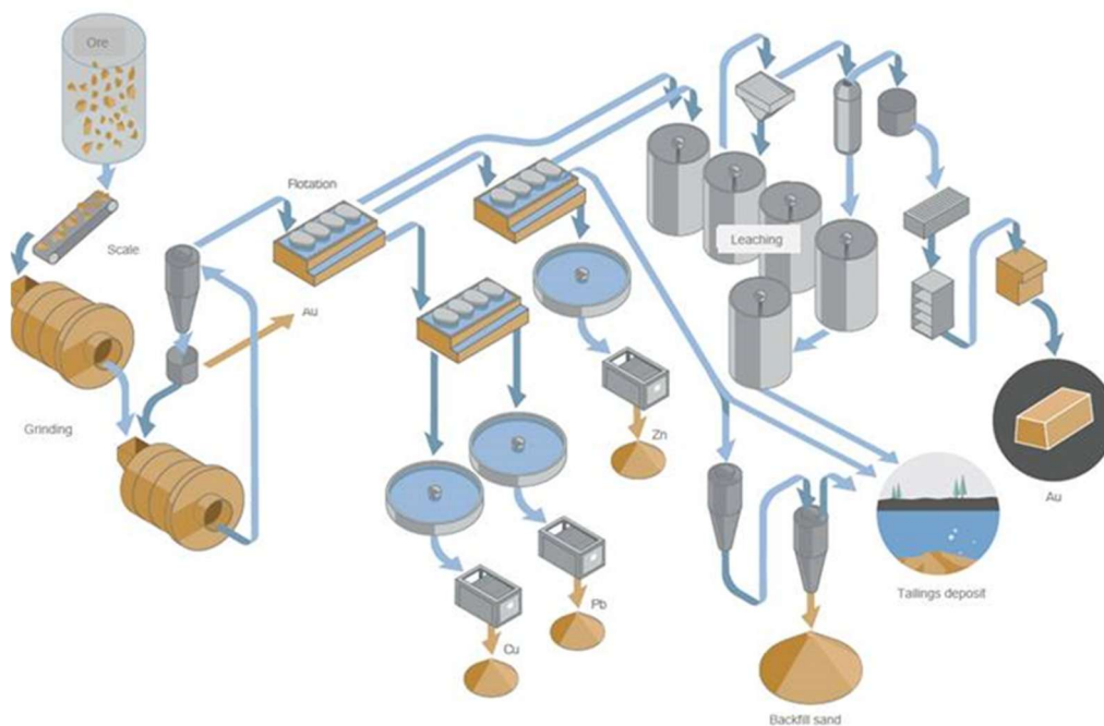
Figure 7: Simplified overview of the different stages of Kristineberg & Rävliiden ore processing at BAOPP
