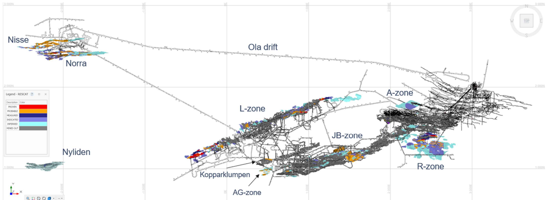
Figure 2: Plan view of the Kristineberg Mine, Rävliiden and Nyliden satellite deposits showing mine infrastructure, historical mined areas and location of Mineral Resources and Mineral Reserves using local grid as reference.
