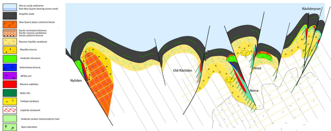
Figure 5: Schematic profile showing the interpreted geological setting of Nyliden in relation to the Rävliiden deposit(s)
