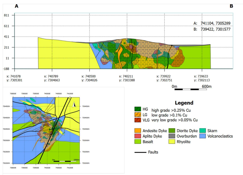
Figure 5. Cross section from SW to NE showing the copper mineralization envelopes relative to the modelled geology.
