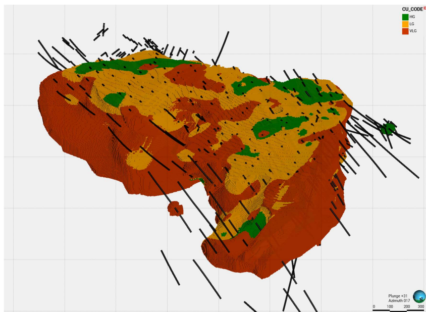
Figure 6. Image of 3D block model coded by Laver mineralization domains with drill hole traces for reference (looking NE, viewed from perspective).
