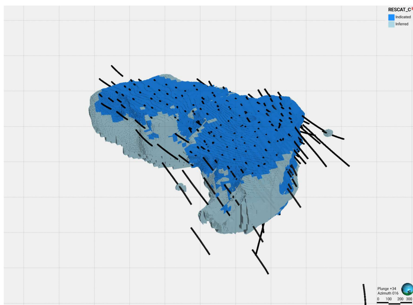
Figure 8. 3D overview showing classification of the Laver mineralization block model; IND – Indicated Resource, INF – Inferred Resource.
