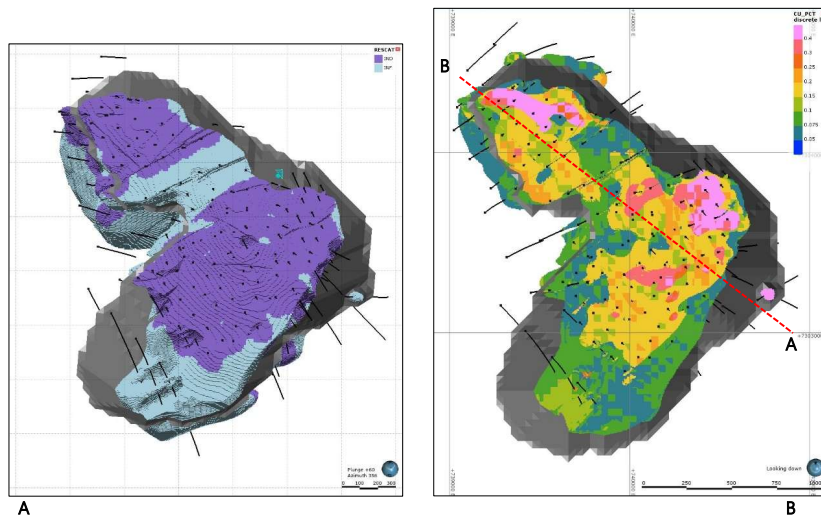
Figure 9. Laver deposit block model; top left) Perspective view of selected resource pit shell with classified mineralization, top right) plan view of selected resource pit shell with Cu grades of mineralization domains and bottom) cross section with unfiltered Cu grades compared against selected resource pit shell.
