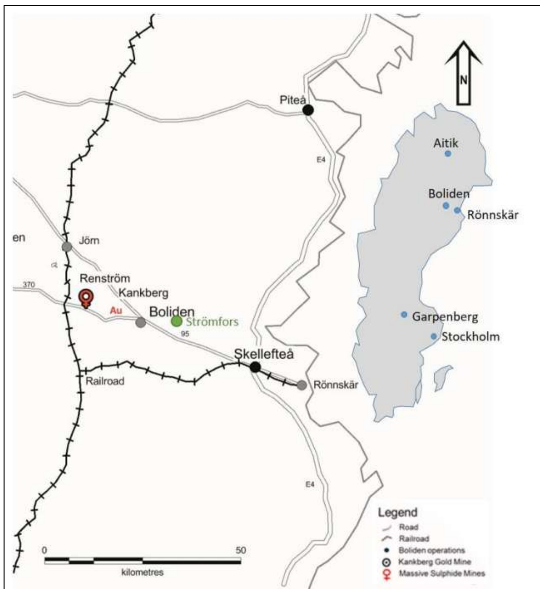
Figure 3.7 Location of the Strömfors project area within the eastern part of the Skellefte mining district in Västerbotten, Sweden. The location of operating mines within the Boliden area (and Sweden) are given for reference.
